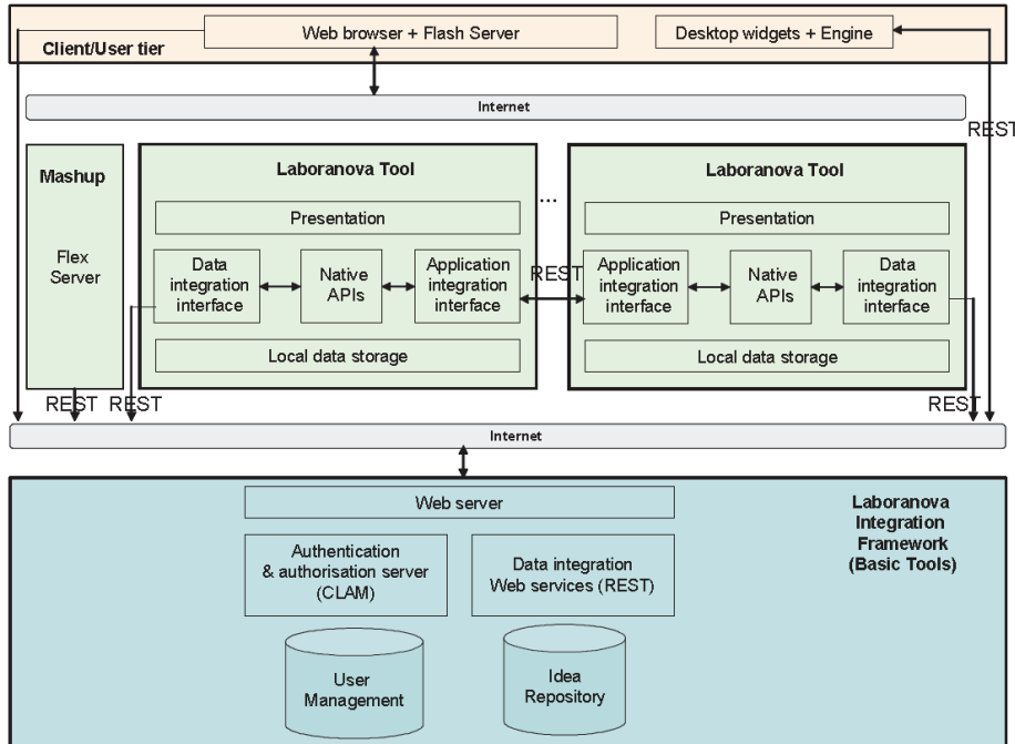
Figure 2. Service-oriented architecture applied to Laboranova. Source: Laboranova project
